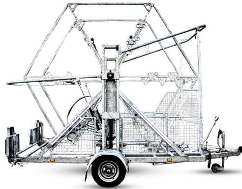
HEXI Pipe Coil Trailer
