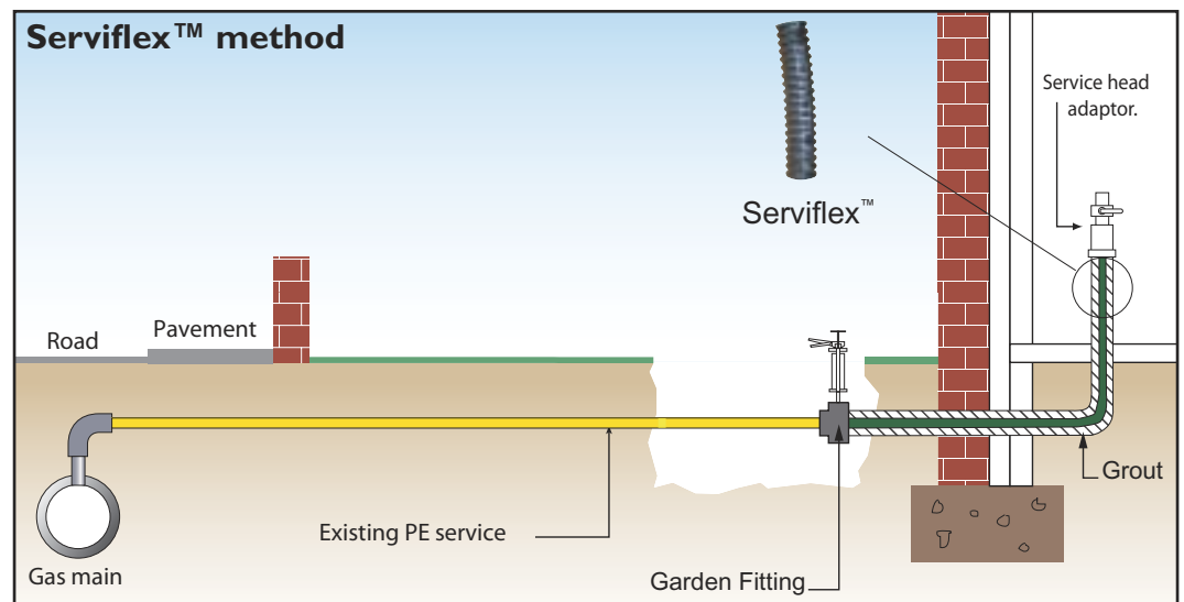
Grout is injected from the garden fitting
