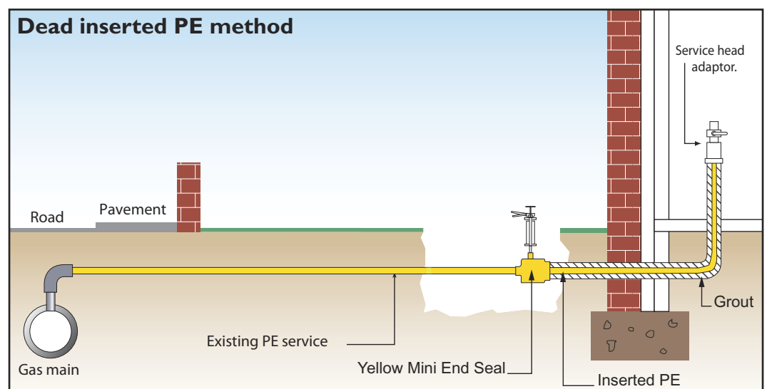
Grout is injected through the yellow mini Endseal™
